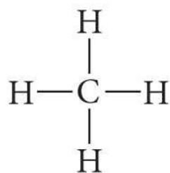
Structural formula
