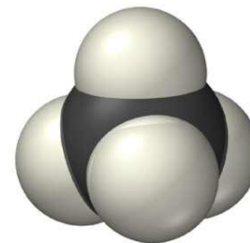
Space-filling model
