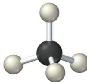
Ball-and-stick model
